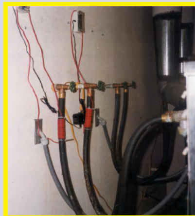
Individual units (pictured to the left) were installed on the hot and cold water lines going to the washing machines (see photograph to the right). The Holiday Inn is saving $4,800 annually on laundry and bleach expenses just from this application alone.
