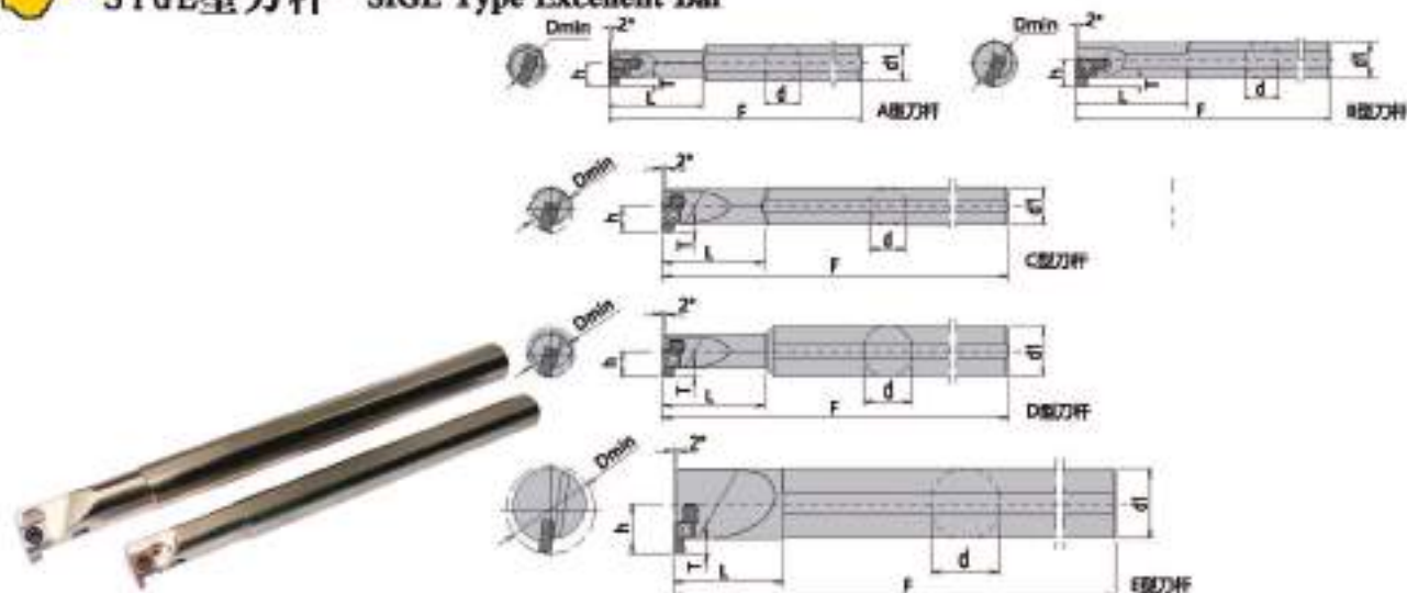
图为右手刀具 Right Cutting Tools(see picture)
