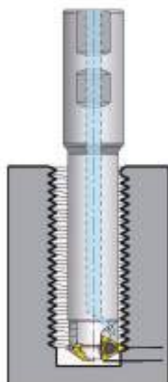
U型适用于大螺距 for large pitches
