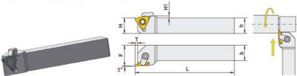
图示为右手刀具 Right Cutting Tools(see picture)
