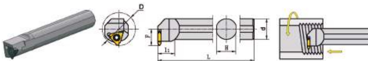
图片为右手刀具 Right Cutting Tools(see picture)
