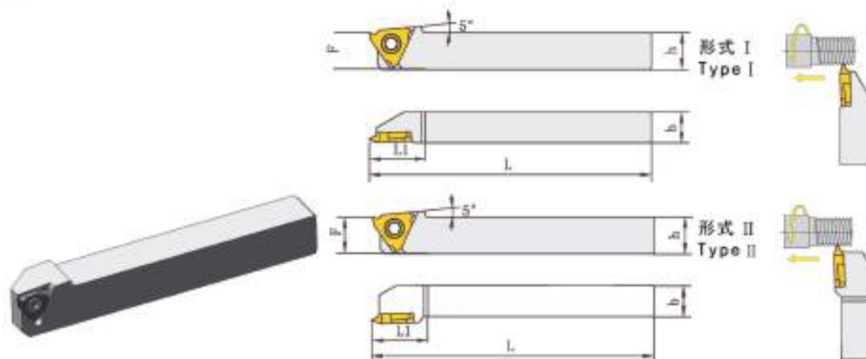
图片为右手刀具 Right Cutting Tools(see picture)
