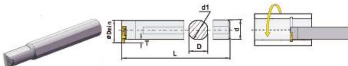
图示为右手刀具 Right Cutting Tools(see picture)
