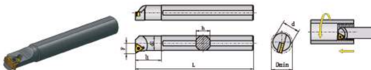
图片为右手刀具 Right Cutting Tools(see picture)
