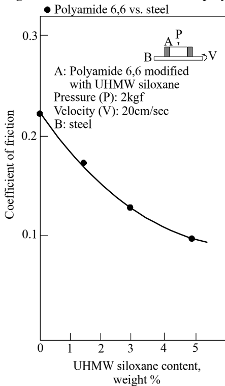
Figure 2: Coefficient of friction of polyamide 6.6 vs. UHMW siloxane content.
