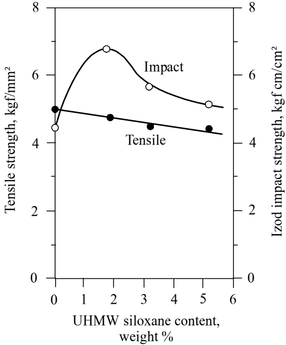
Figure 1: Effect on physical properties of polyamide 6.6.
