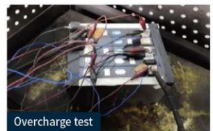
Overcharge test
