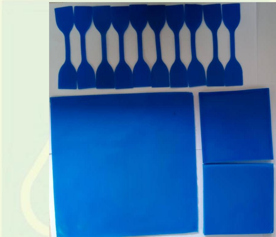
Figure 1. Photograph of PVC WATERSTOP; Brand: "UniStop" Test Specimens
