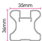
Vertical Frame (Left & Right)
