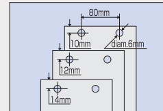
DEPTH GAUGE
