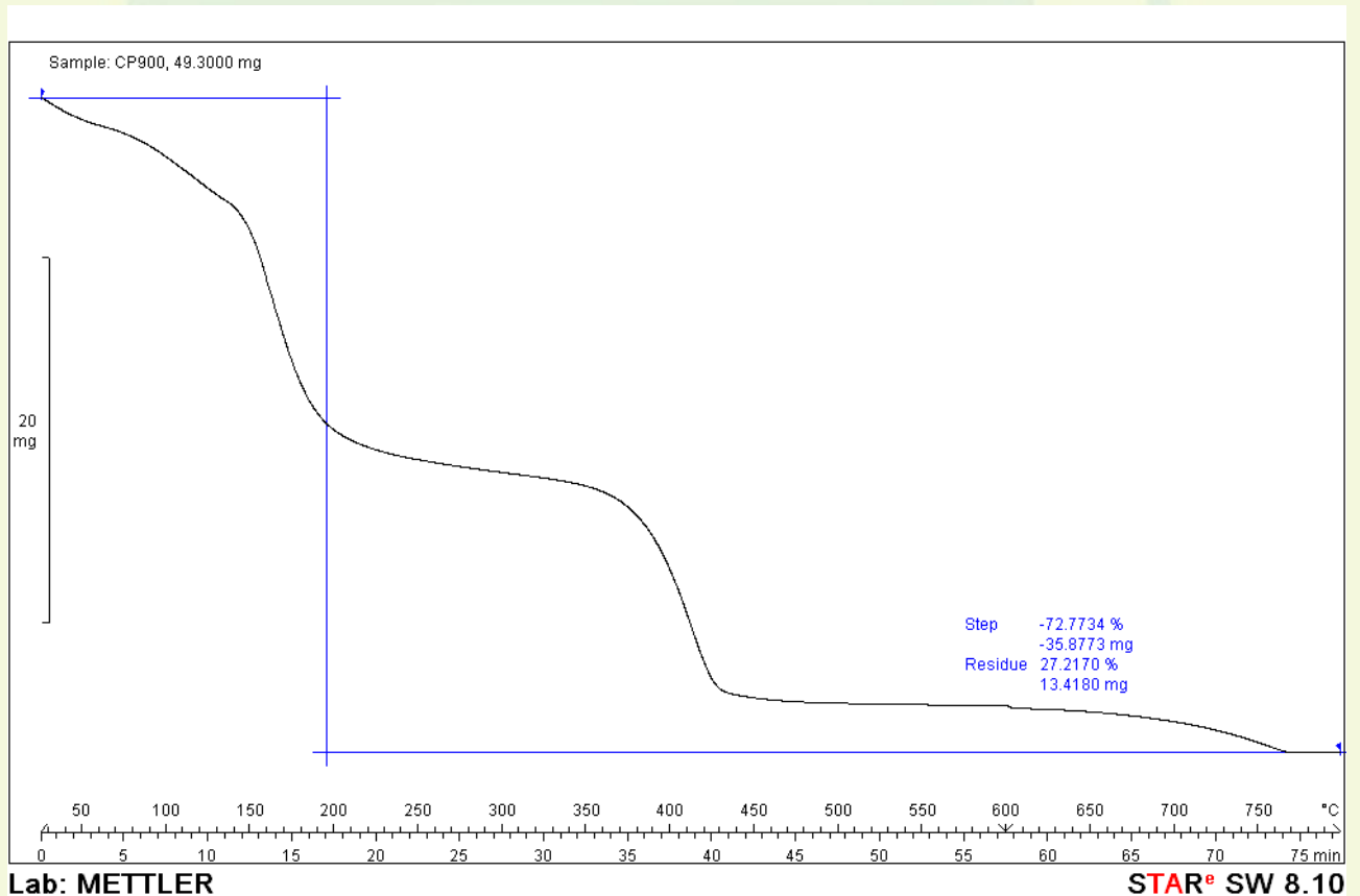
Figure A.1. TGA Curve of 'DRI-GARD CF 900; Brand: DRITECH' Sample
