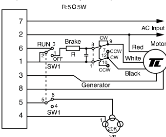
SS31/SS32 (R) 速度控制正逆轉加電子剎車接線圖 SS speed control with electronic brake (Bi Directional Operation)
