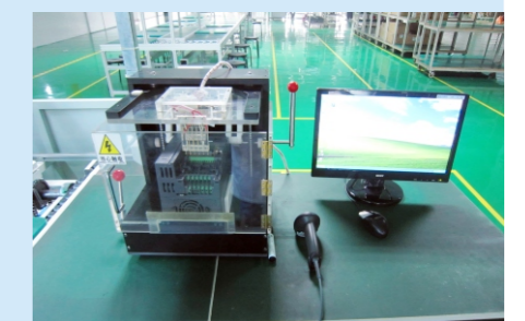
Automatic FLASH test platform
