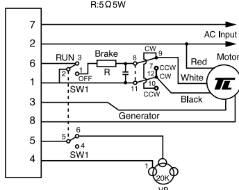
SS31/SS32 (R) 速度控制正逆轉加電子剎車接線圖 SS speed control with electronic brake (Bi Directional Operation)
