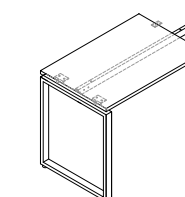
PX3 SR960 Side Return L900 * W600 * H750mm
