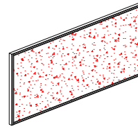
Desktop Screen (Full Fabric) with White Aluminium Frame PX FF900 - L 900 * H700 * T23mm PX FF1000 - L1000 * H700 * T23mm PX FF1200 - L1200 * H700 * T23mm PX FF1300 - L1300 * H700 * T23mm PX FF1500 - L1500 * H700 * T23mm
