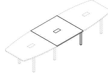
PX5 REC1200 Rectangular Extension Conference Table with 1 U-Hollow Metal Leg L1200 * W1200 * H750mm
