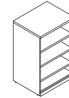
PX5 MHC1370 Medium Height Open Shelf Cabinet L800 * W400 * H1370mm
