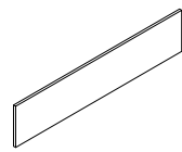
Wooden Modesty Panel + Hanging Bracket (2pcs) PX5 MP1200 - L 800 * W300 * T18mm PX5 MP1400 - L1000 * W300 * T18mm PX5 MP1500 - L1100 * W300 * T18mm PX5 MP1600 - L1200 * W300 * T18mm PX5 MP1800 - L1400 * W300 * T18mm
