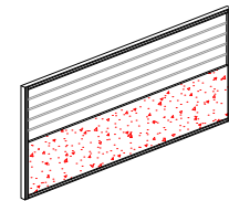
Desktop Screen Half Fabric & Half Polycarbonate (Brown + White Aluminium Frame) PX HF900 - L 900 * H700 * T23mm PX HF1000 - L1000 * H700 * T23mm PX HF1200 - L1200 * H700 * T23mm PX HF1300 - L1300 * H700 * T23mm PX HF1500 - L1500 * H700 * T23mm
