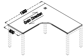
PX5 1515T Universal WorkTop L1500/600 * W1500/600 * T25mm
