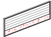
Desktop Screen with 1/3 Fabric & 2/3 Polycarbonate (Brown + White Aluminium Frame) PX SC900 - L 900 * H530 * T23mm PX SC1000 - L1000 * H530 * T23mm PX SC1200 - L1200 * H530 * T23mm PX SC1300 - L1300 * H530 * T23mm PX SC1500 - L1500 * H530 * T23mm
