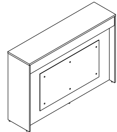
PX5 RC18 Reception Counter L1843 * W420 * H1135mm
