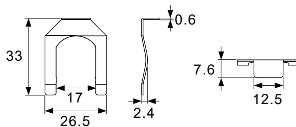
C-clip
