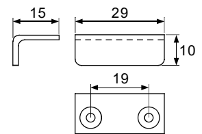
Striking Plate
