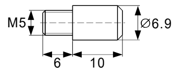
Extension Pin
