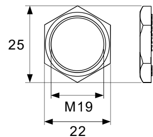
Hexagon Nut
