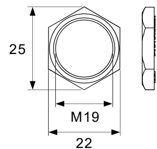
Hexagon Nut
