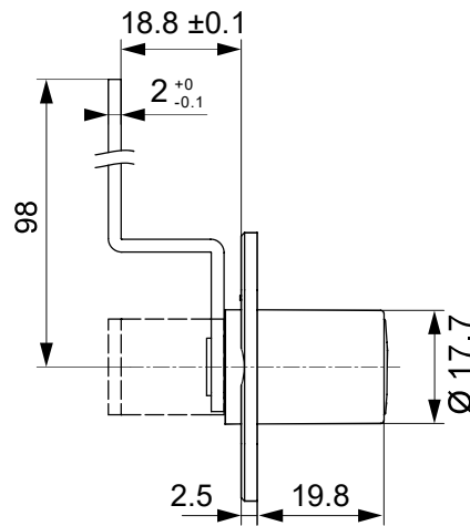
Bracket
