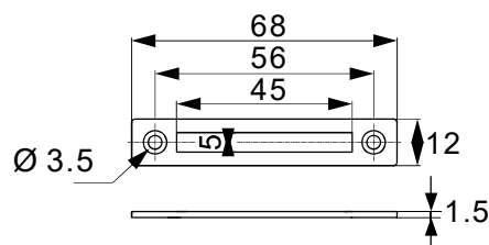
Striking Plate
