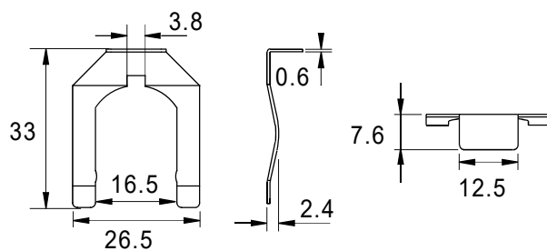
C-Clip
