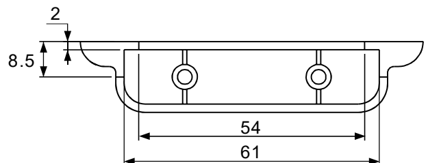
Part for Double Door
