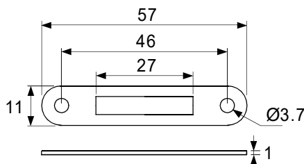
Striking Plate
