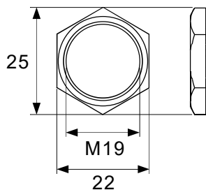
Hexagon Nut
