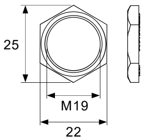
Hexagon Nut
