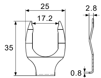
C-clip
