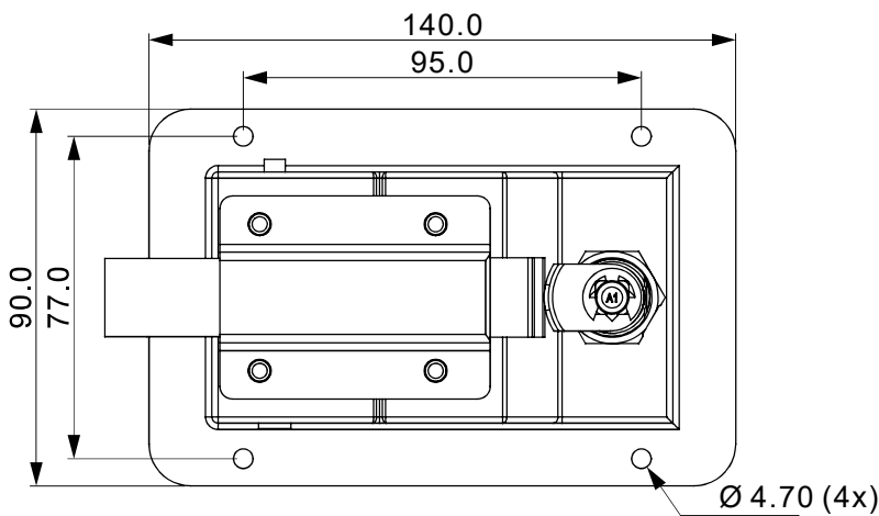
Food Truck, Caravan Car, etc
