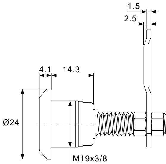
Locker, Cupboard, etc
