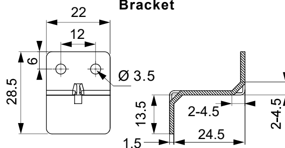
Bracket
