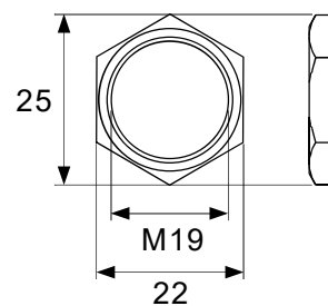
Hexagon Nut
