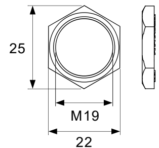
Hexagon Nut
