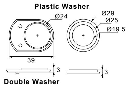
Double Washer
