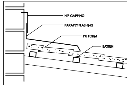
FLASHING
