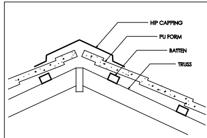
HIP CAPPING
