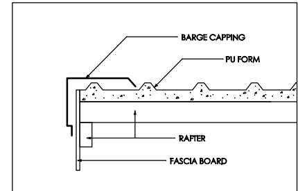
BARGE CAPPING
