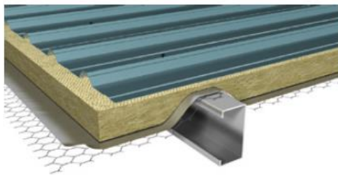
Single Skin Roof System
