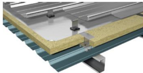
Double Skin Roof System
