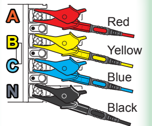
For a bus bar, pinch the metal part.
