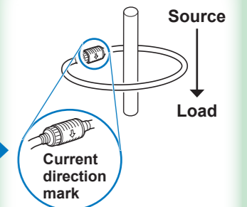
Attach the sensor around only one of the conductor.
