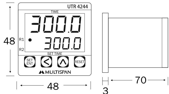
Outline Dimension (mm)
