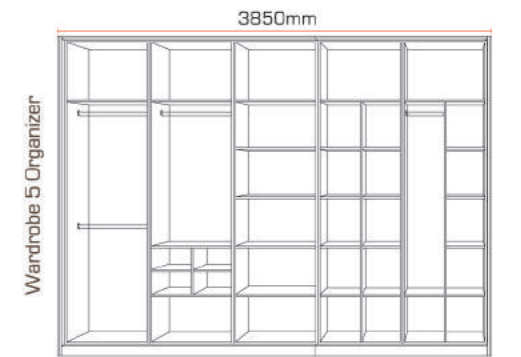
For width: 762mm x 5 Organizer = 3810mm + 40mm [side panel x 2] = 3850mm
