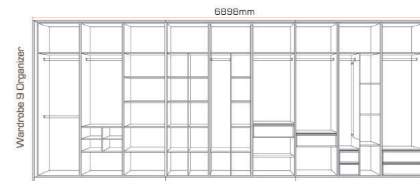
For width: 762mm x 9 Organizer = 6858mm + 40mm [side panel x 2] = 6898mm
