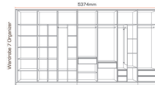
For width: 762mm x 7 Organizer = 5334mm + 40mm [side panel x 2] = 5374mm
