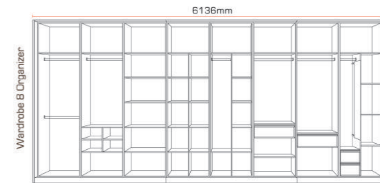
For width: 762mm x 8 Organizer = 6096mm + 40mm [side panel x 2] = 6136mm
