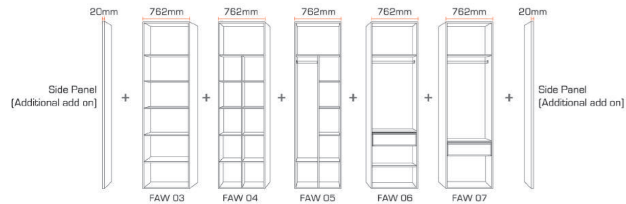
For width: 762mm x 5 Aluminium Organizer = 3810mm + 40mm [side panel x 2] = 3850mm Standard Height: 2438mm
