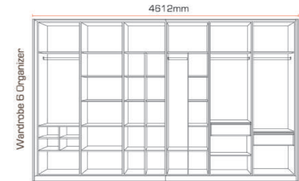
For width: 762mm x 6 Organizer = 4572mm + 40mm [side panel x 2] = 4612mm
