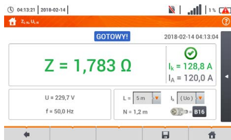
Fault loop impedance measurement
