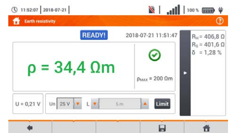
Ground resistivity measurement
