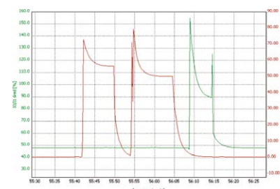
Example of asymmetry caused by connection process
