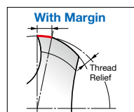
Con-Eccentric Thread Relief
