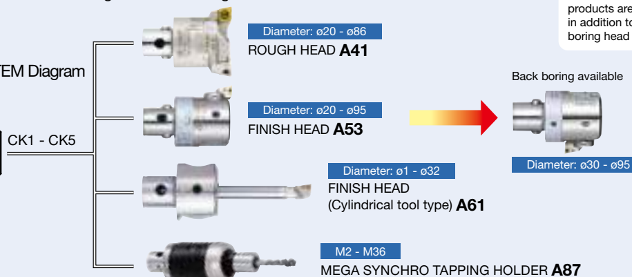
HSK-F Type
