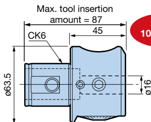
Head EWN2-50CK6
