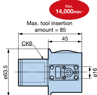
Head EWE2-54CK6
