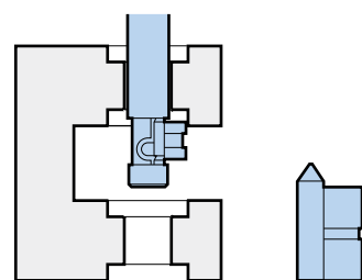
Wing for front and back spot facing
