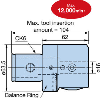
Head EWB2-50CK6
