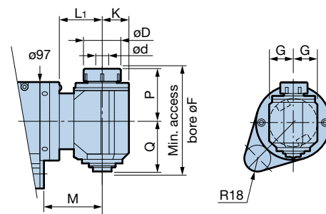
Fig. 4 High Rigidity Type Max.3,000min -1
