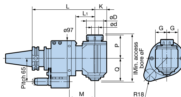
Fig. 3 High Rigidity Type Max. 3,000min -1
