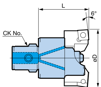
A Type for Through-Holes
