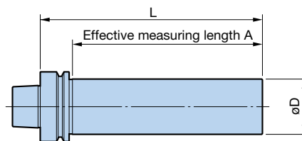
HSK-F Type (DIN 69893-6)
