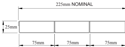
UNDERFLOOR TRUNKING (STANDARD 25mm TRUNKING HEIGHT)
