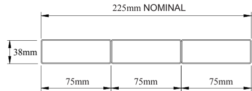
uPVC TRUNKING (STANDARD 75mm X 38mm)
