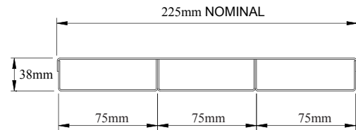
UNDERFLOOR TRUNKING (STANDARD 38mm TRUNKING HEIGHT)
