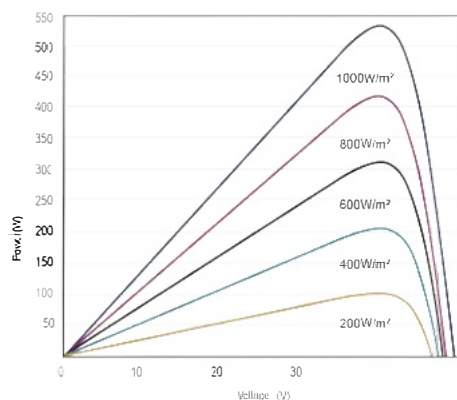
P-V CURVES OF PV MODULE(540W)
