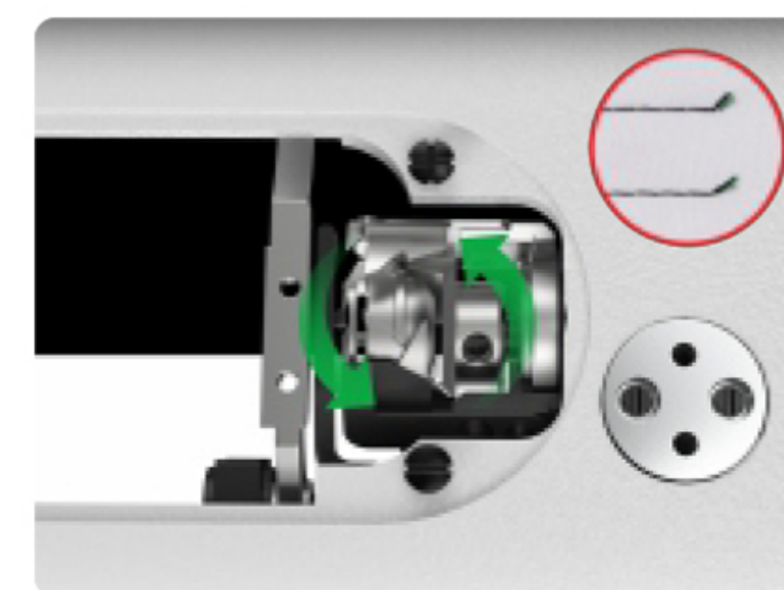
双刀剪线：短线头 Double blade thread cutting: Short thread end
