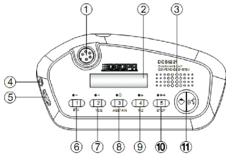
Top view of delegate unit
