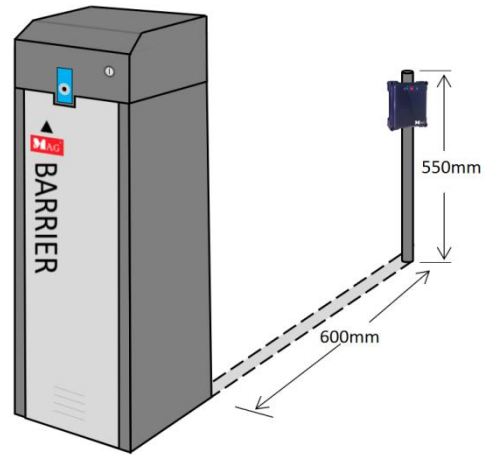
Example traffic detector install separately on a metal pole
